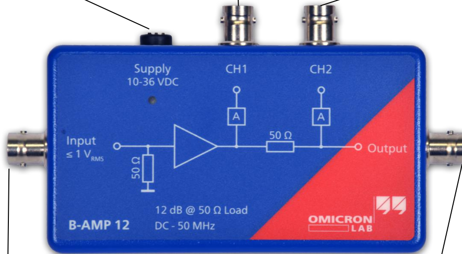
Figure 3-1: B-AMP 12 connector description
